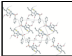
Fig. 2. The packing and hydrogen bonding of (I) viewed down b axis. Hydrogen atoms not involved in the showed interactions have been omitted for clarity.
